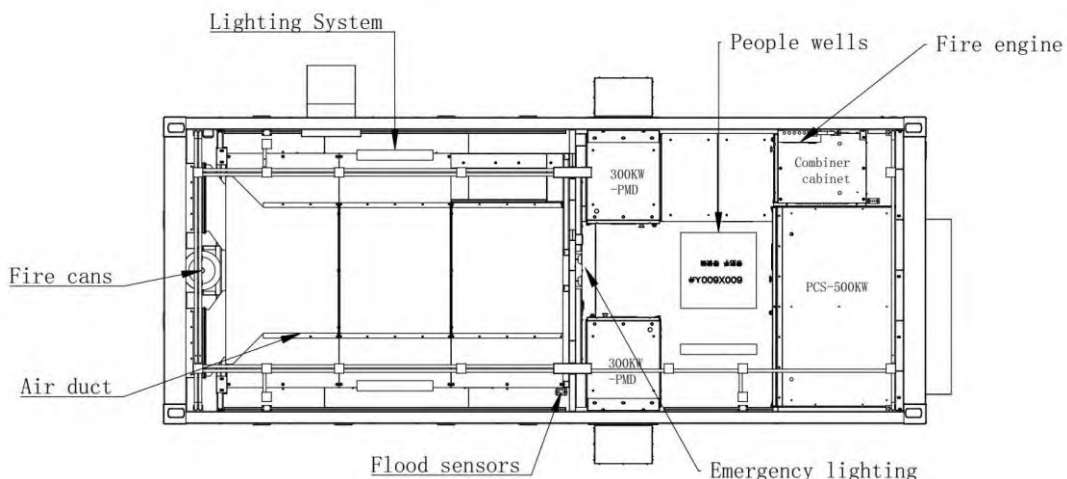
Configuration within the 20 feet container system
