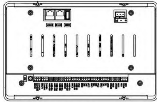
ES-01 Rear Terminal
